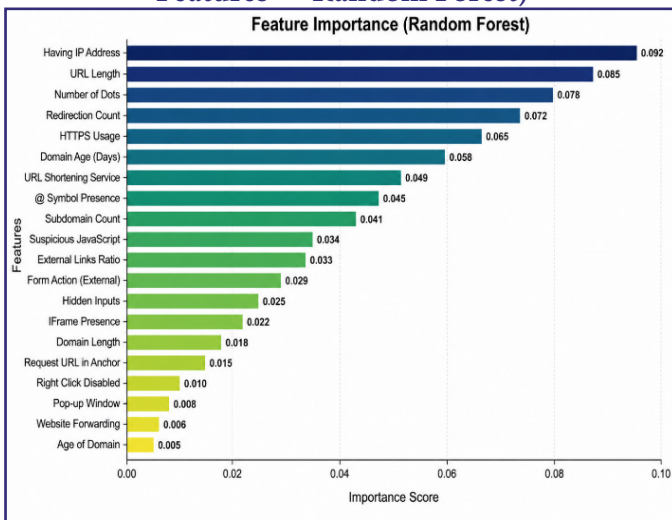
Fig. 2: Feature Importance Graph (Top 12 Features — Random Forest)
