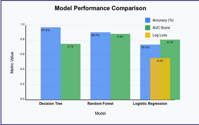
Fig. 6: Model Performance
