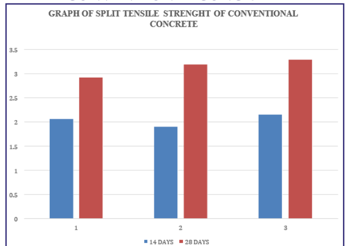
GRAPH 03: SPLIT TENSILE STRENGHT OF CONVENTIONAL CONCRETE
