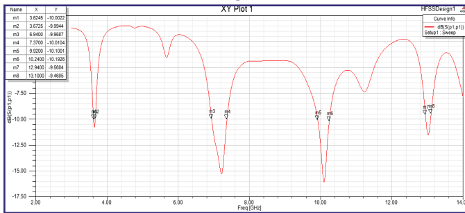
Fig. 3: Return loss vs. frequency of V slot MSA
