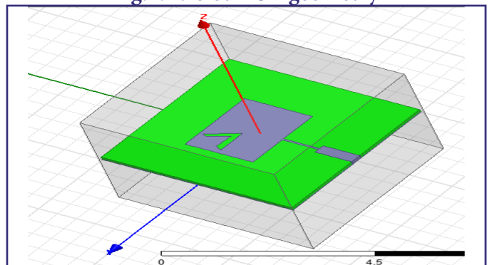
Fig.2. V slot MSA geometry
