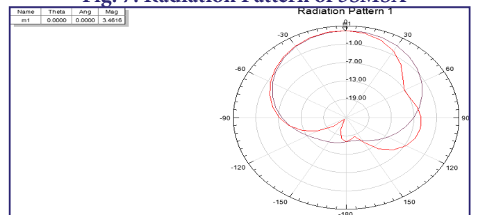
Fig. 7: Radiation Pattern of 5SMSA
