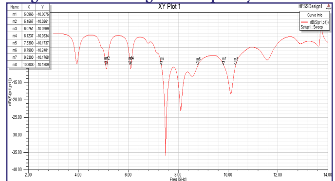
Fig. 6: Return loss against frequency of 5SMSA
