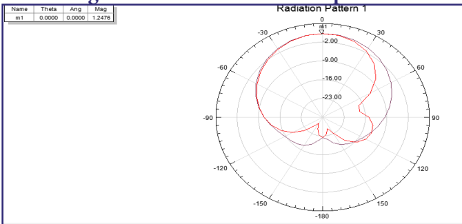
Fig. 4: V-slot MSA radiation pattern
