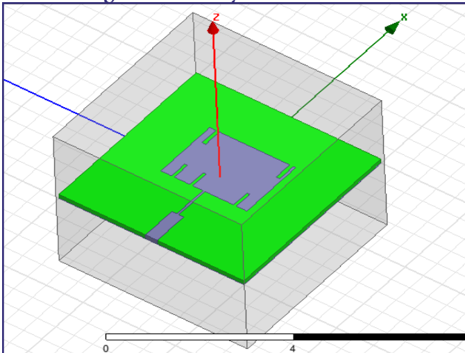
Fig. 5: Geometry view of 5SMSA
