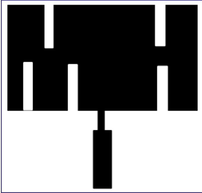
Fig. 1(a): Conventional Microstrip Antenna
