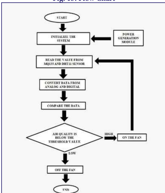
Fig. 13: Flow Chart
