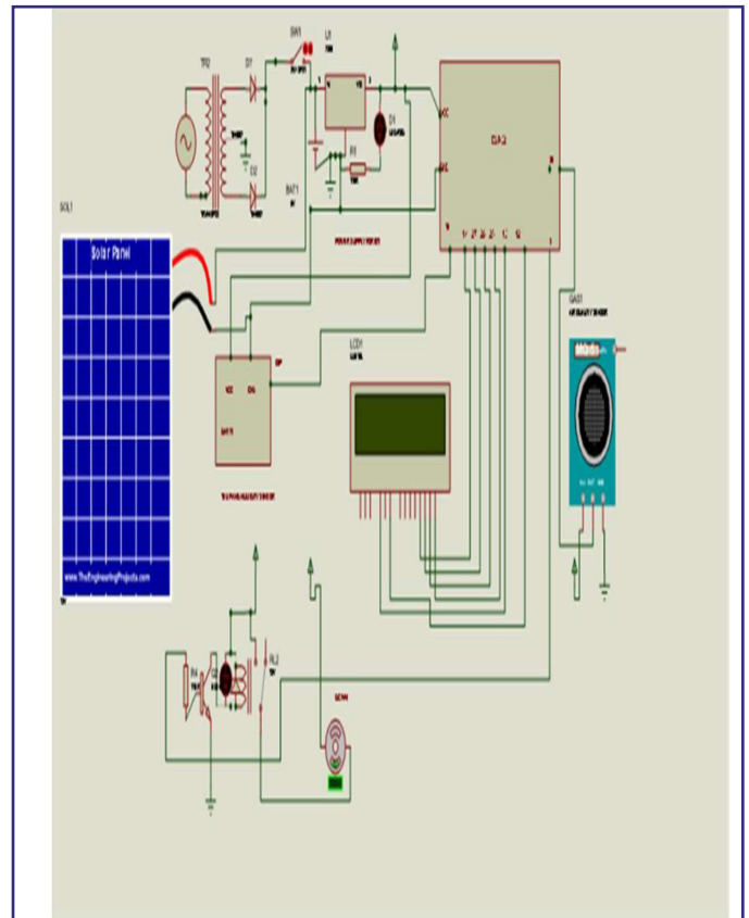
Fig. 12: Circuit Diagram: Solar Powered Air Purifier
