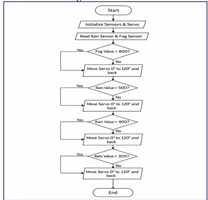
Fig. 9: Flow Chart
