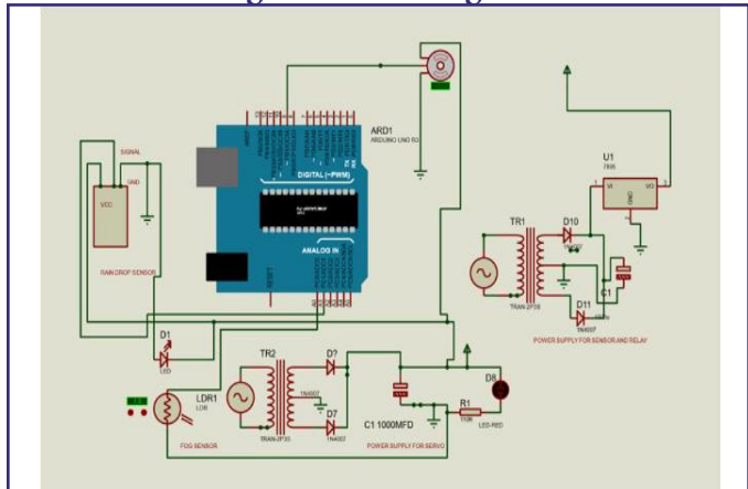
Fig. 8: circuit diagram
