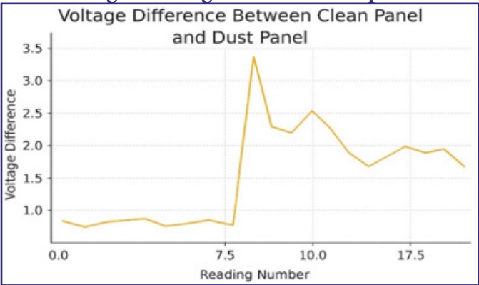
Fig. 6: Voltage Difference Graph
