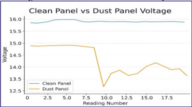
Fig. 5: Clean Panel vs Dust Panel Graph
