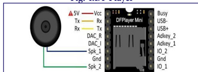
Fig. 4:DF Player
